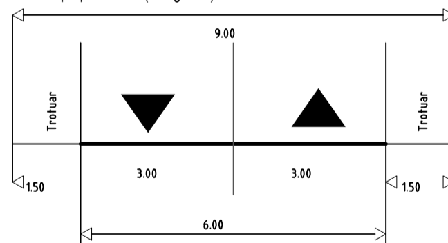
Profil propus - T1-4 (categ. III.1)
