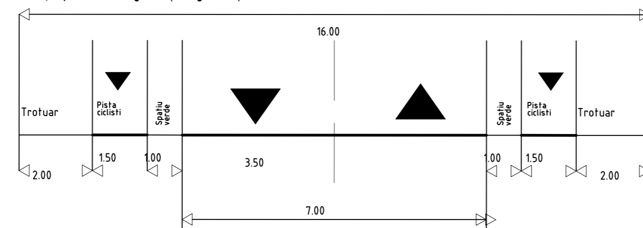
Profil propus - Bd. Magheru (categ. III.6b)
