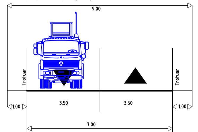
Profil propus - T1-9 (categ. III.1)
